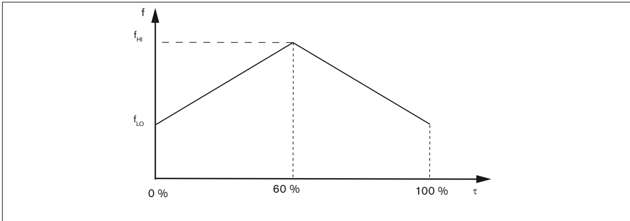
Figure 17: PWM frequency / pulse duty factor
