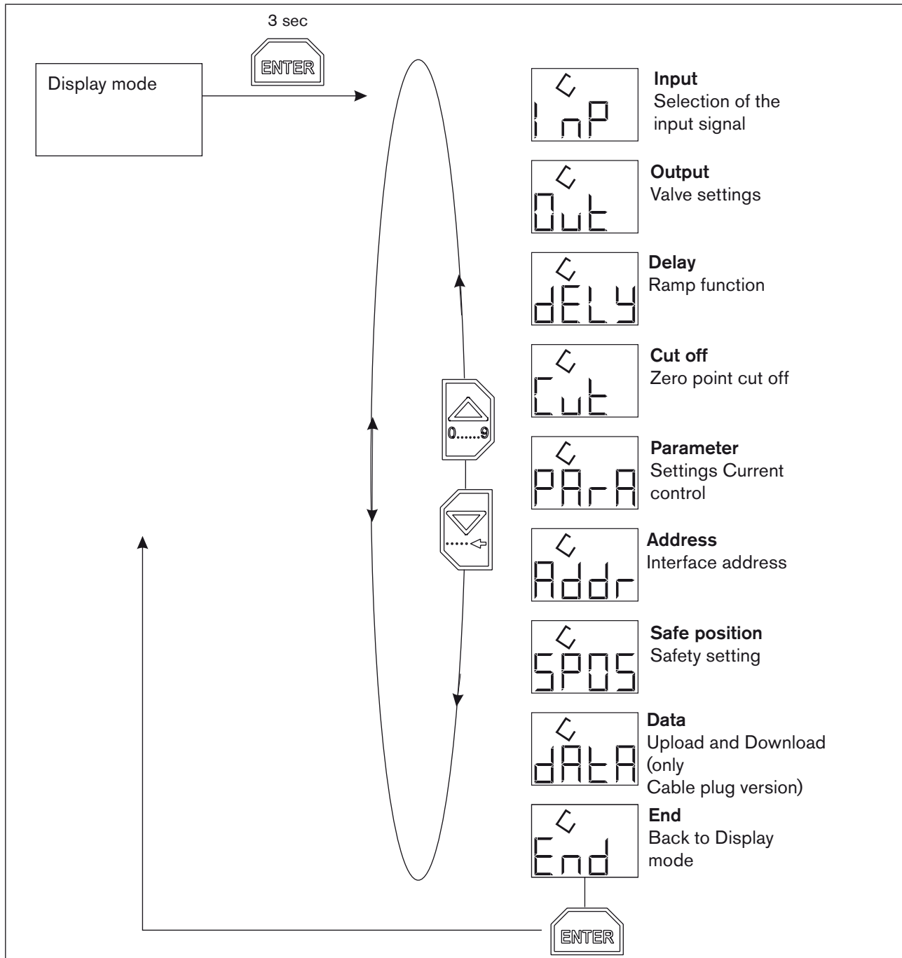
Figure 14: Menu of the configuration mode
