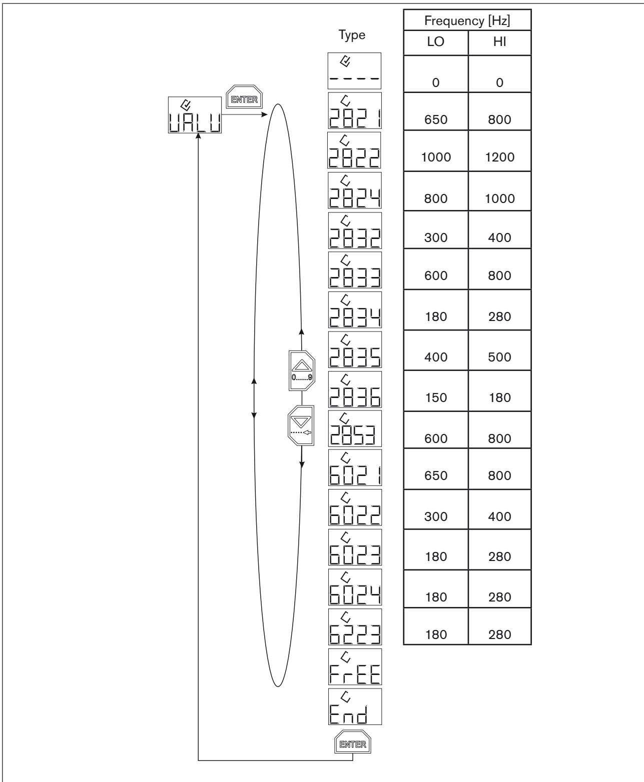
Figure 18: Limit frequencies for Bürkert valve types
