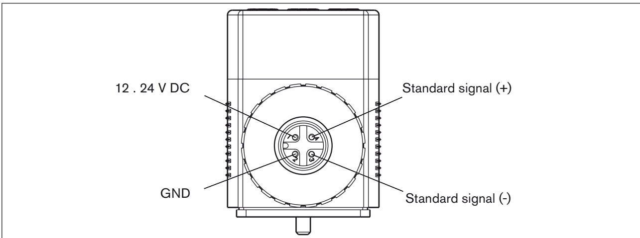
Figure 10: Plug connector connection
