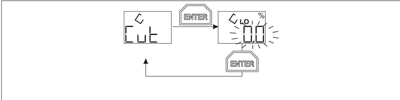
Figure 22: Cut (Cut off) - Zero point cut off
