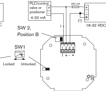
Fig. 3.12 Pin assignment, Position B
