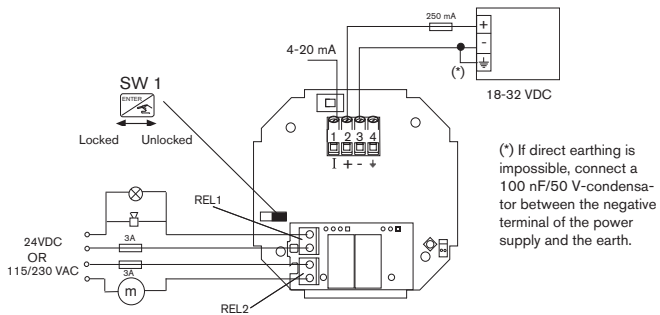
Fig. 3.17 Pin assignment for relays
