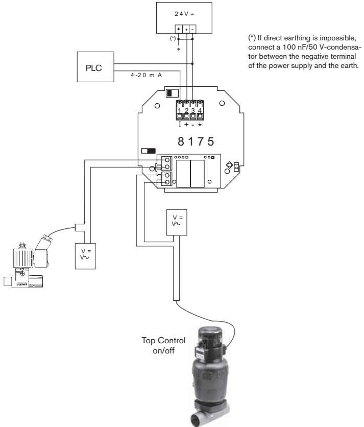
Connection example between the 8175 level transmitter 18-32VDC and the 8631 Top Control on/off mounted on a diaphragm valve 2031 and pilot valve 6012.
