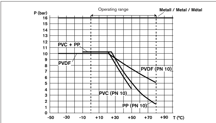
Fig. 3.1 Temperature-pressure dependence
