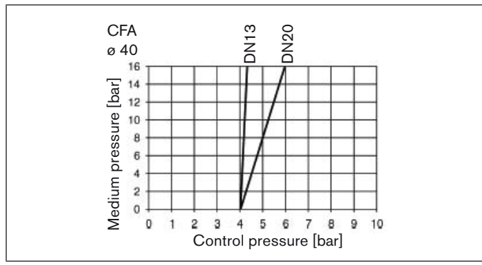
Fig. 12: Pressure graph, actuator ø 40, control function A
