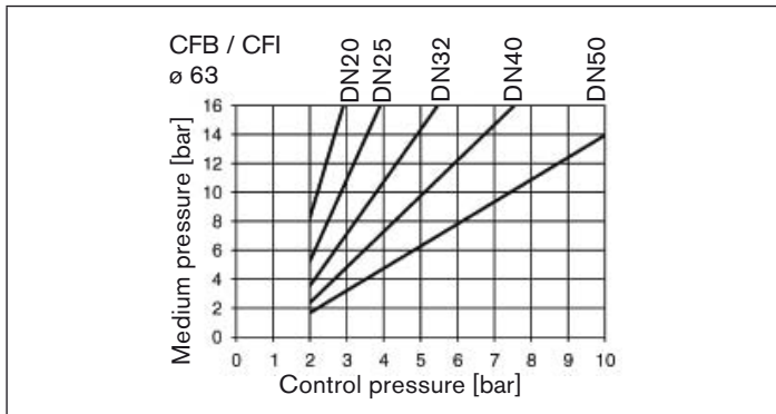
Fig. 8: Pressure graph, actuator ø 63, control function B and I
