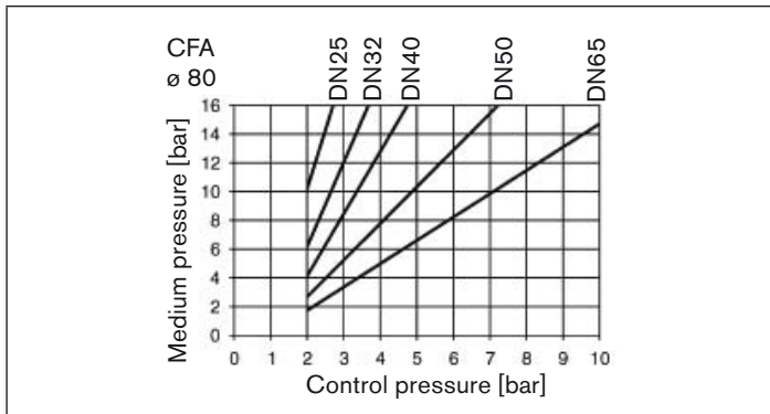
Fig. 15: Pressure graph, actuator ø 80, control function A
